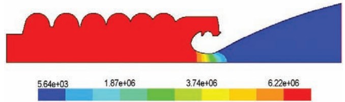
Figure 13. Contours of static pressure at 10 s.
