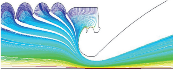
Figure 15. Streaklines in the flow at 10 s configuration.
