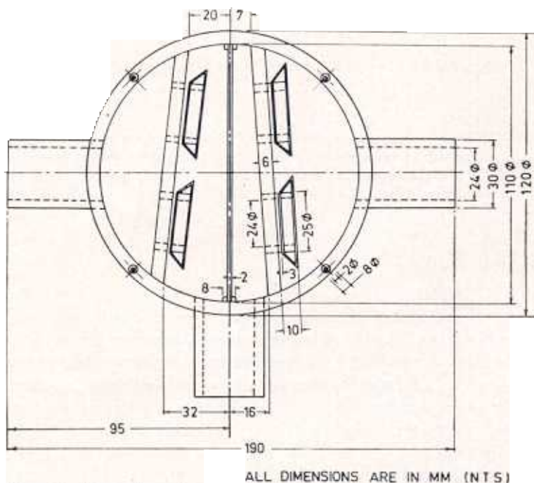
Figure 1. Respiratory valve
