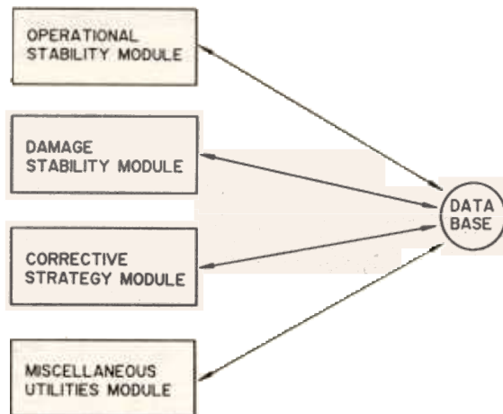
Figure 3. Program modules.
