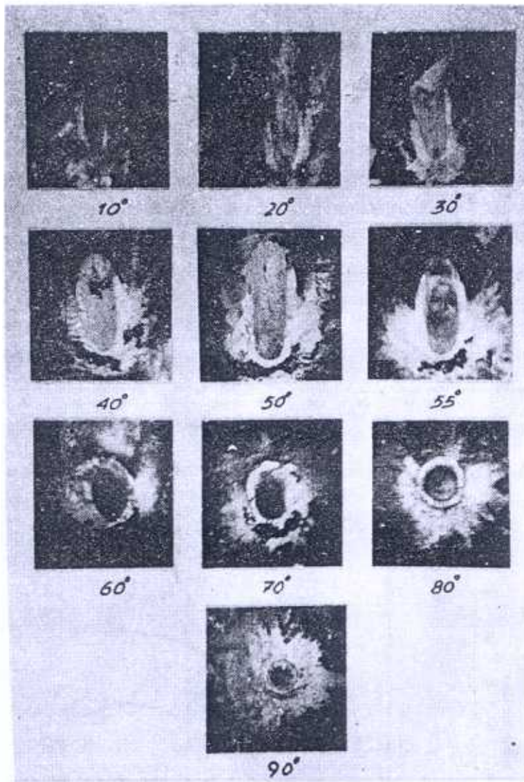
Figure 2. Damage incultated on 55 mm hard steel plate at different angles of impact by 30 mm AP shots.
