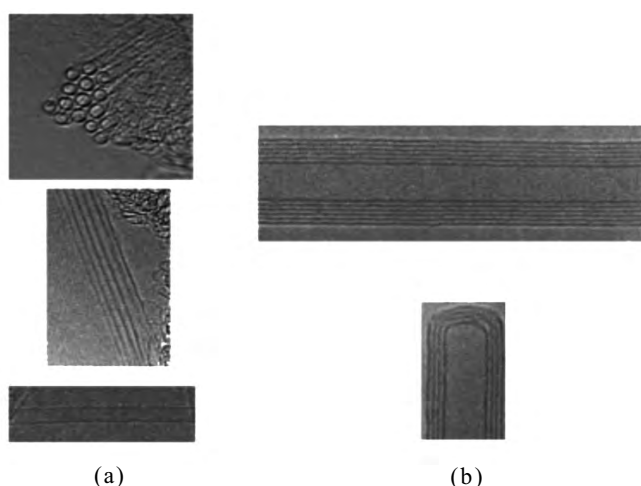
Figure 4. (a) HRTEM image showing the SWNT in bundles, (b) HRTEM images of a MWNT along its length and at the end.
