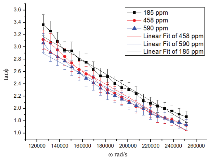
Figure 5. Linear fit decay time plots between tangent of phase and modulation frequencies of laser diode from 20 kHz to 40 kHz for Nitrogen Dioxide gas on different concentrations at 50 mbar pressure.
