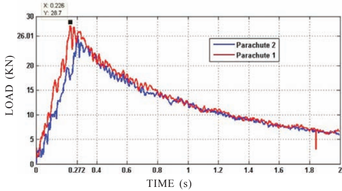
Figure 3. Measured load profile of the parachutes.
