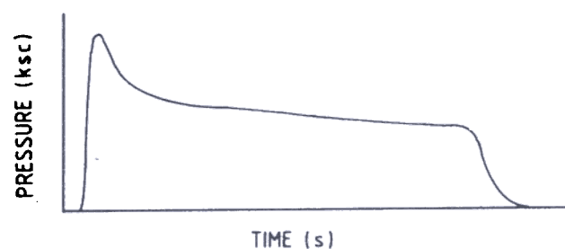
Figure 2. Ballistic output of composition with stable combustion.
