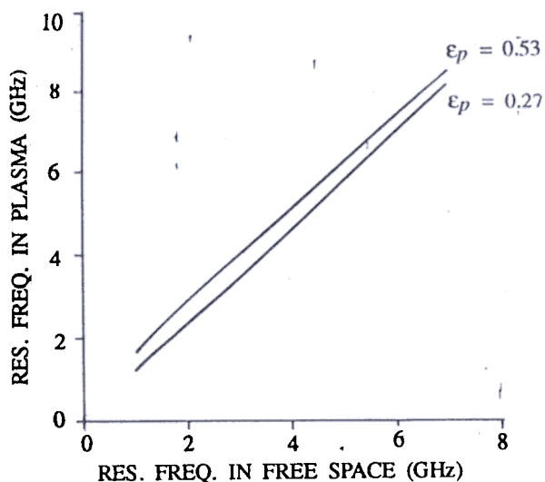
Figure 3. Comparison of resonant frequencies in plasma with that in free-space ( L is varied, to vary the free-space resonant frequency).
