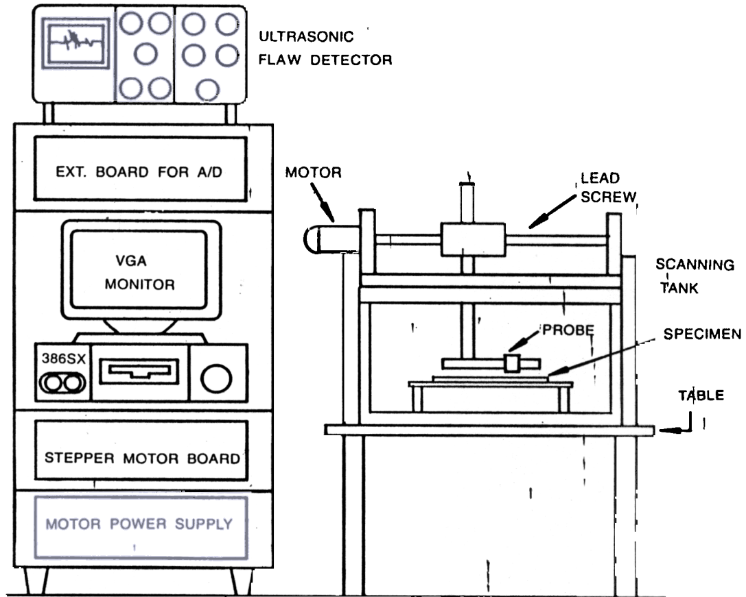
Figure 1. Schematic diagram of automated ultrasonic C-scan system
