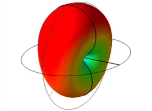
Figure 3. The simulated 3D radiation pattern of the designed antenna.
