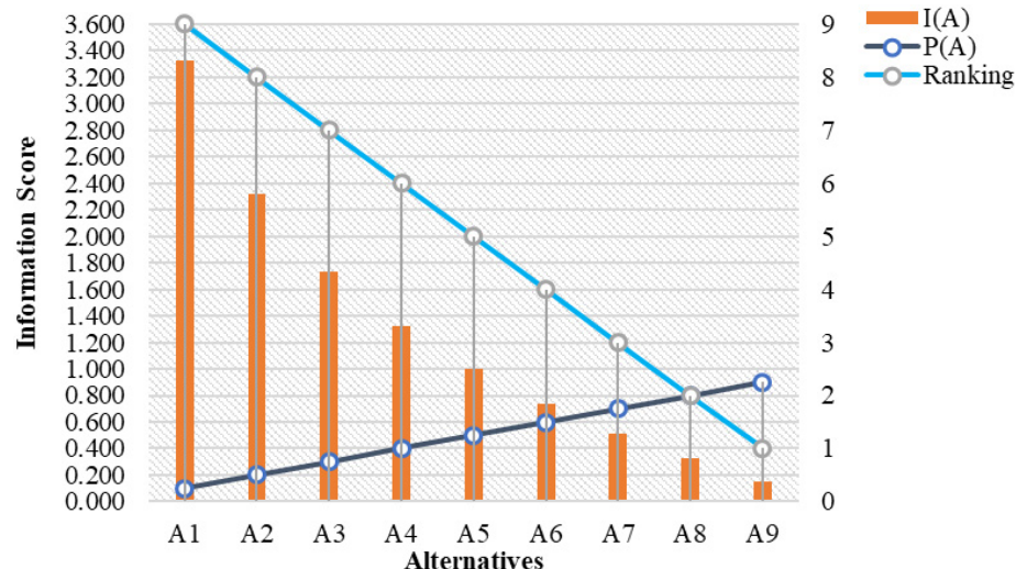
Figure 1. The relation between probability and the amount of information.
