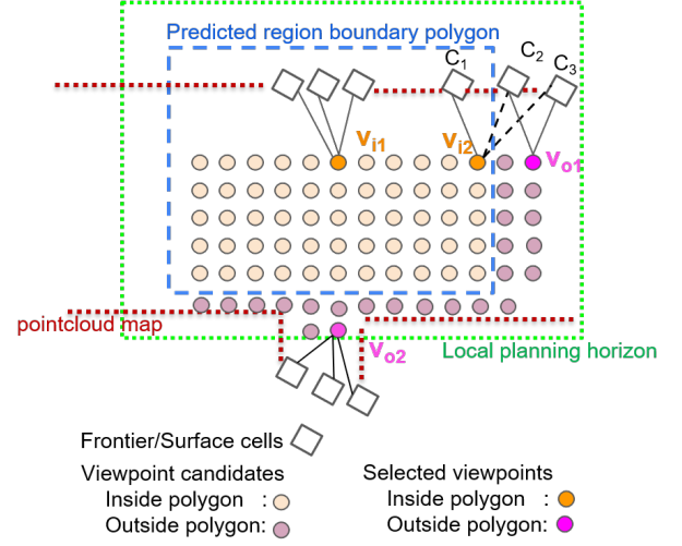
Figure 3. The figure shows the visibility of frontier cells from viewpoints. The dashed edges show the visibility of cells outside the predicted region boundary by viewpoint v_{12} .
