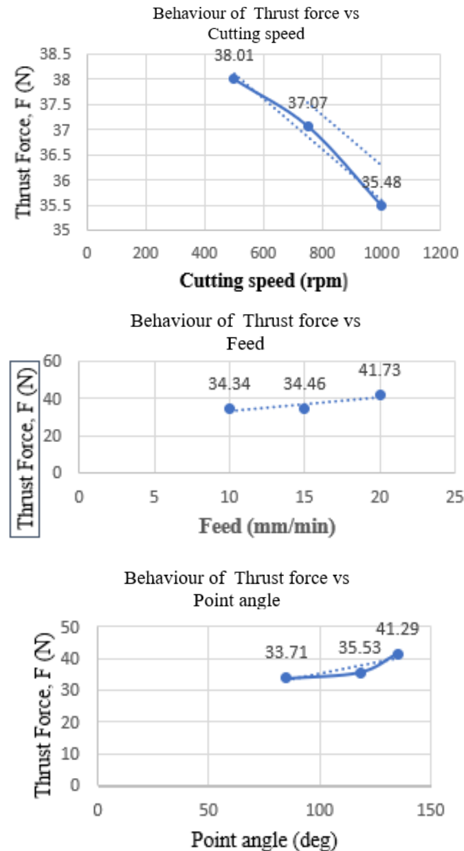
Figure 4. Cutting parameters versus thrust force.
