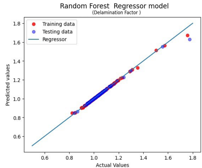
Figure.7 Actual Vs predicted delamination-RF.
