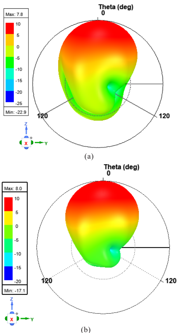
Figure 6. Far-field gain pattern of the proposed antenna (a) without DGS; and (b) with circular slot DGS.
