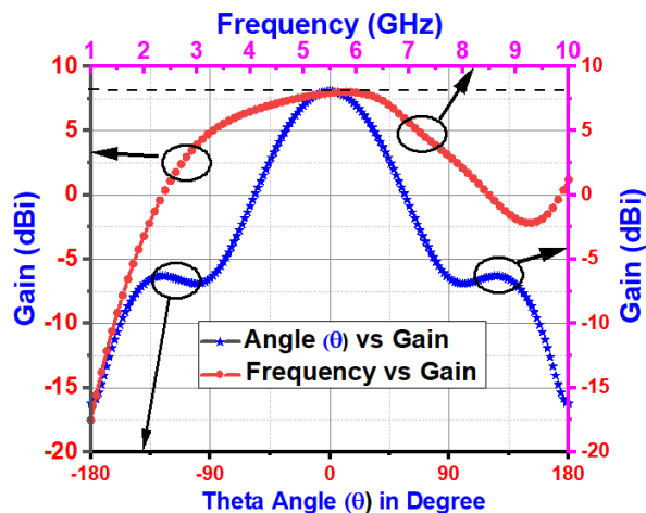
Figure 5. Gain versus frequency and gain variation for different theta angles.
