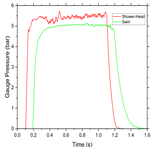
Figure 9. Pressure time curve with gaseous oxygen only for both injectors.
