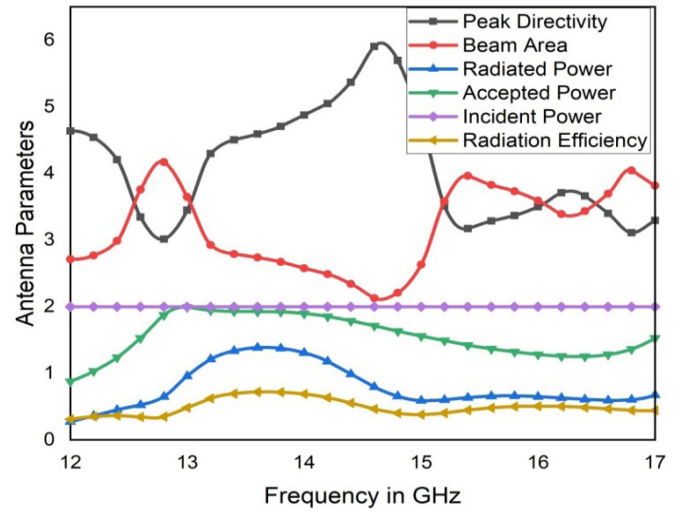
Figure 12. Performance of other antenna parameters.
