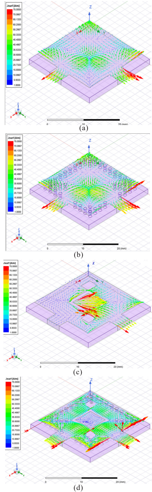
Figure 4. Current distributions of development steps of proposed antenna design, (a) Step-1: Antenna without SIW and slots (b) Step-2: Antenna with SIW; (c) Step-3: Antenna with slots; and (d) Step-4: Antenna with SIW and slots (proposed).
