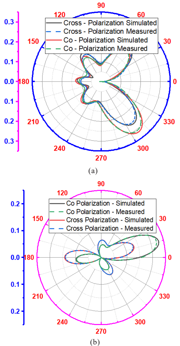
Figure 10. E Plane and H Plane radiation pattern, Co polarization and cross polarization pattern (both simulated and measured) of proposed DA, (a) at 13 GHz; and (b) 14.625 GHz.
