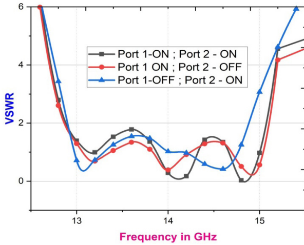
Figure 7. VSWR of proposed diplexing antenna (DA).
