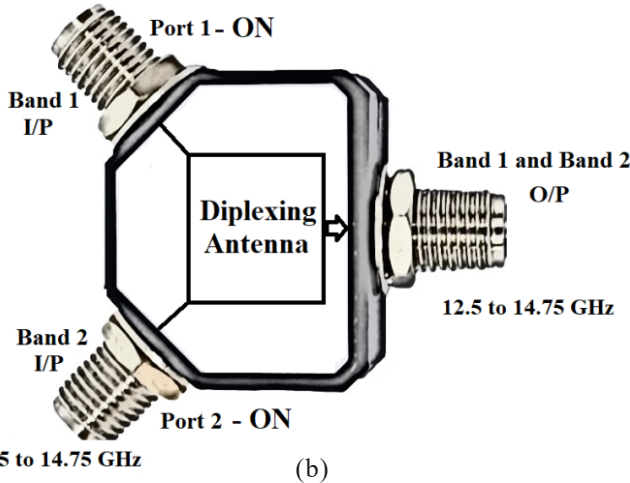
Figure 1. (a) Frequency requirement of ITU-R recommendation of DR satellite low and medium data rate for uplink; and (b) Diplexing antenna operation.
