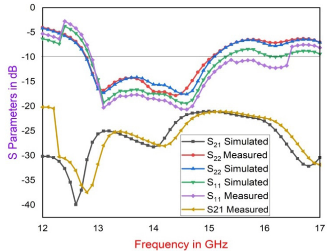
Figure 13. Simulated and measured reflection coefficients.
