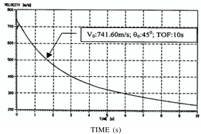
Figure 5. Velocity versus time plot for shot-1 (S-1) by measurement.
