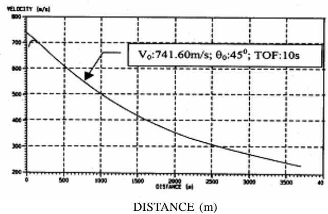
Figure 6. Velocity versus distance plot for shot-1 (S-1) by measurement.
