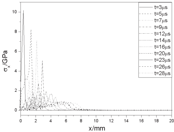
Figure 2. Stress \sigma_x versus position x at different time.
