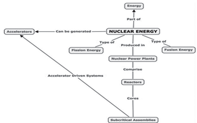
Figure 5. Nuclear energy.
